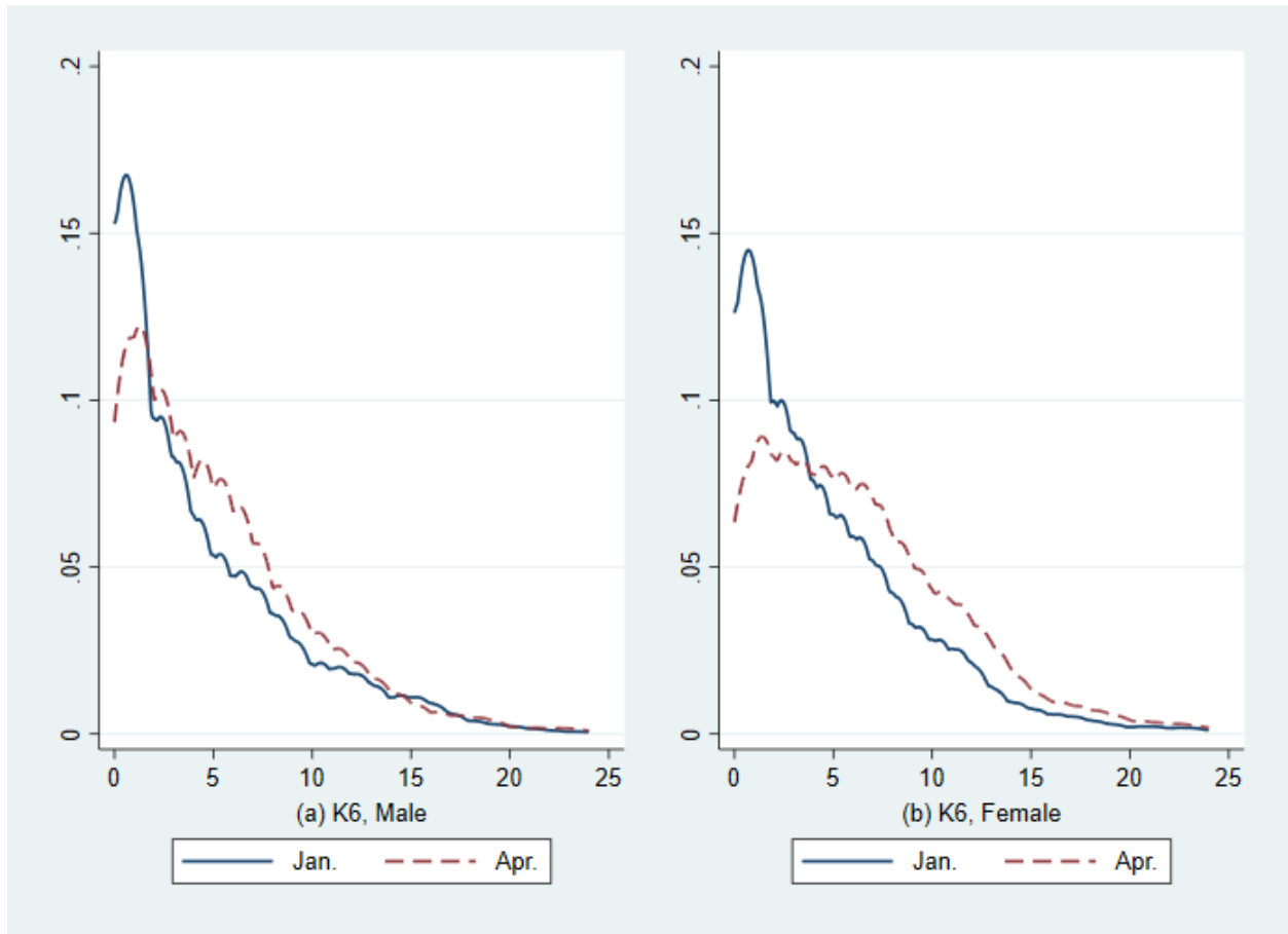
Figure 1: Distributions of K6 scale in January and April
